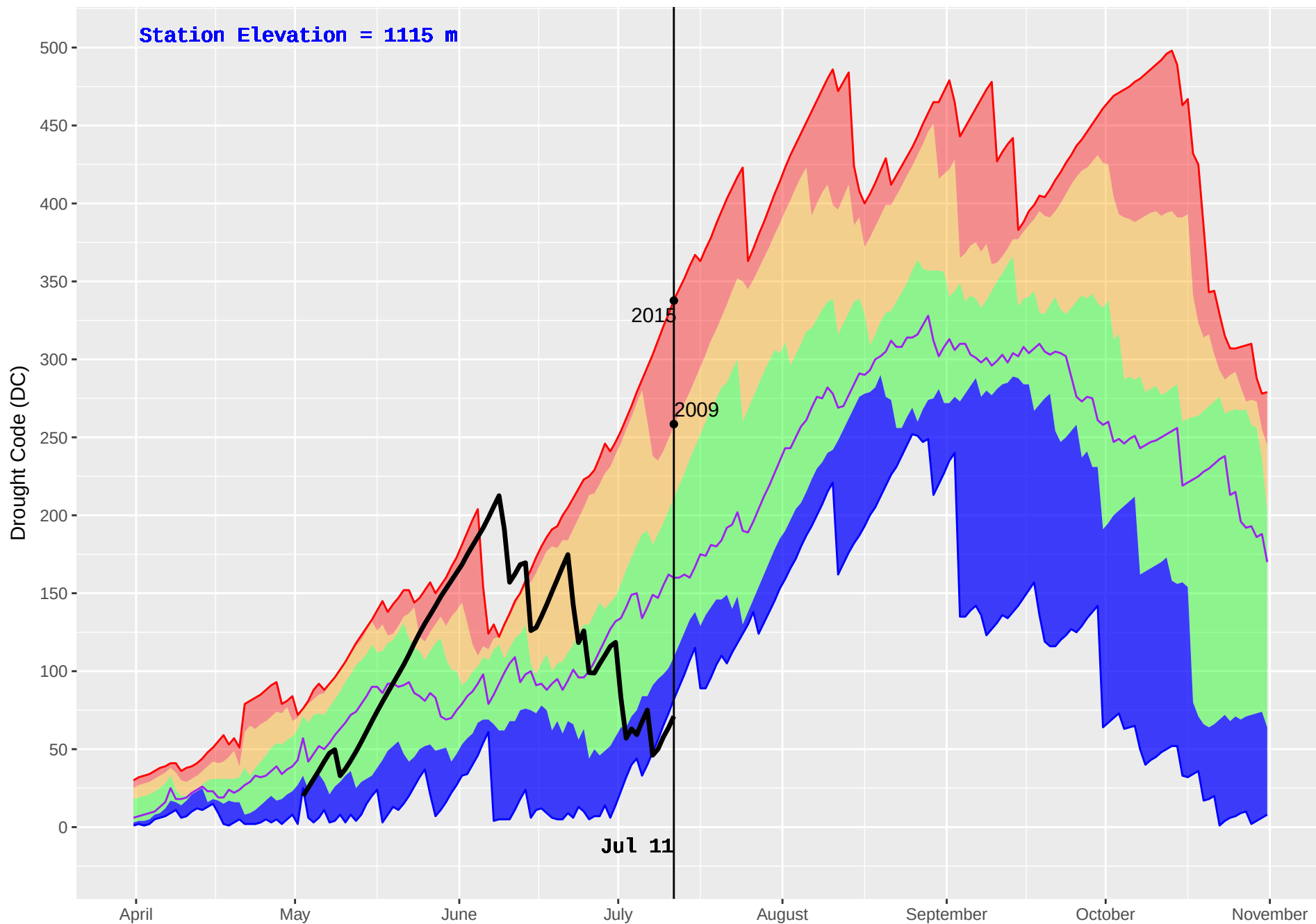
SICAMOUS (882) : Historical (2004–2016) and Current (2018) Noon Drought Code (DC)
