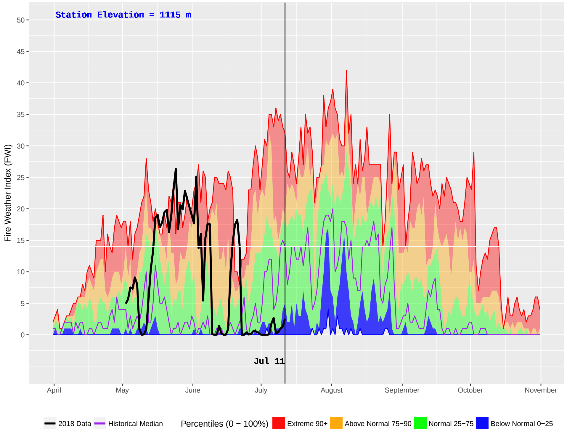
SICAMOUS (882) : Historical (2004–2016) and Current (2018) Noon Fire Weather Index (FWI)
