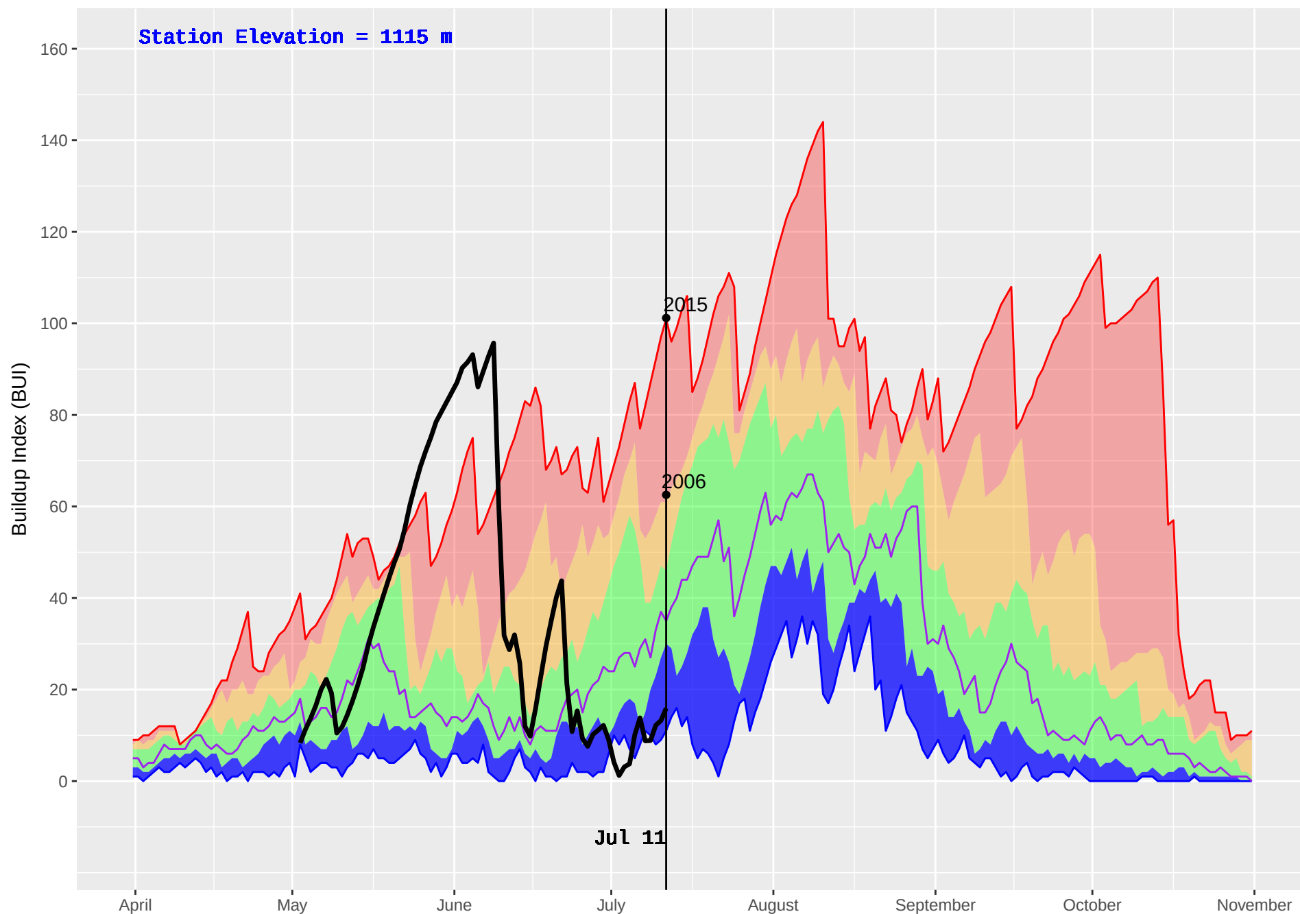
SICAMOUS (882) : Historical (2004–2016) and Current (2018) Noon Buildup Index (BUI)
